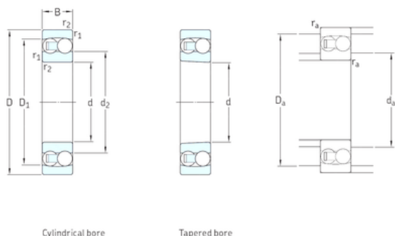
Cylindrical bore
